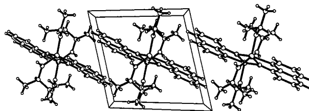
Fig. 5 Crystal packing diagram of [(t\text{Bu})_2\text{Al}(\mu\text{-O}-8-\text{C}_9\text{H}_6\text{N})_2] 5 .
