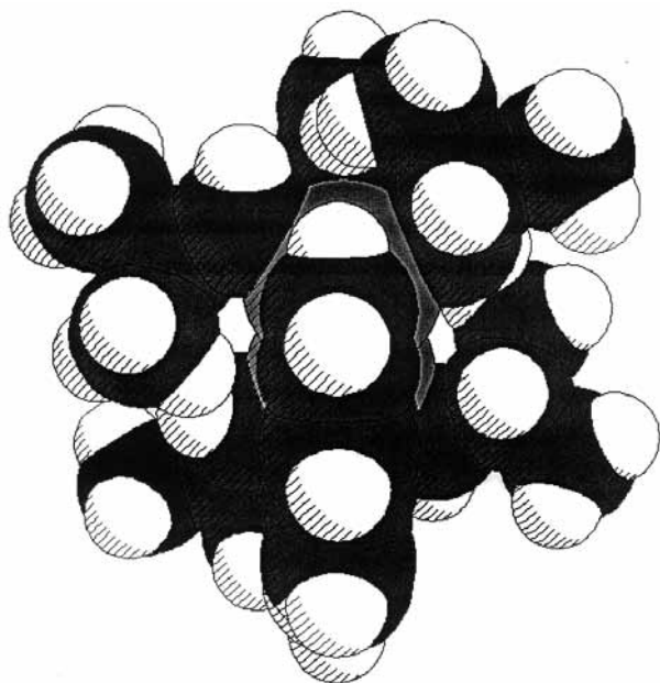
Fig. 7 Space filling diagram of [(t\text{-Bu})_2\text{Al}(\mu\text{-O-8-C}_9\text{H}_6\text{N})]_2 5 , showing the anti arrangement of the isobutyl groups.
